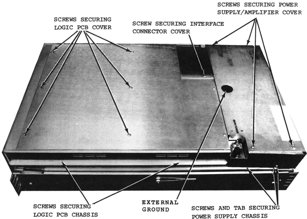
Figure 3-1. Cover Removal
