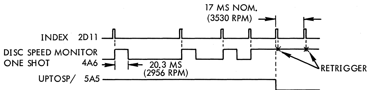
Figure 4-34. Up-To-Speed Detection
