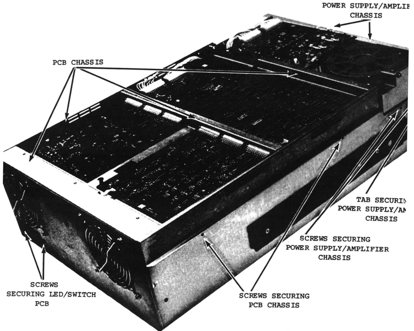
Figure 5-14. REFLEX II Front/Side View
