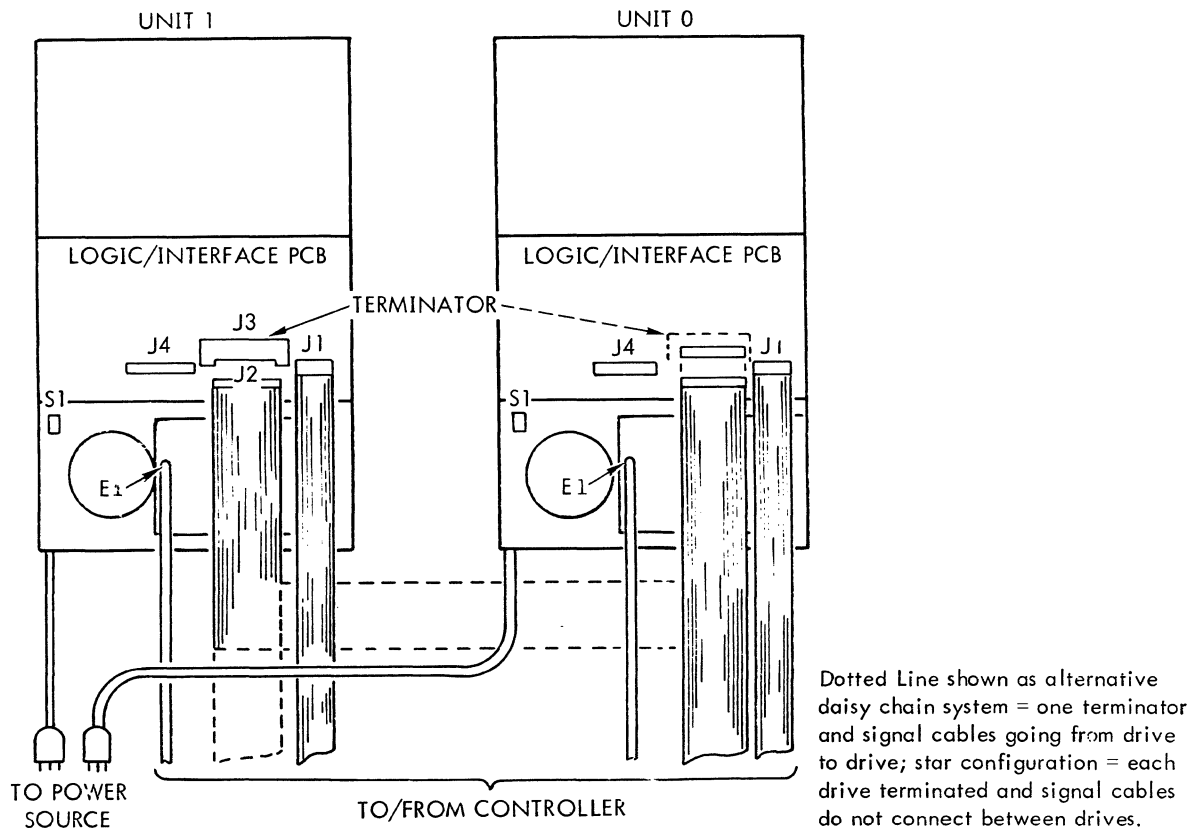
Figure 3-6. Cable Connections
