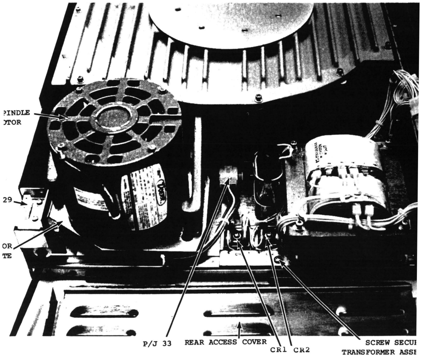
Figure 5-16. Reflex II Rear View
