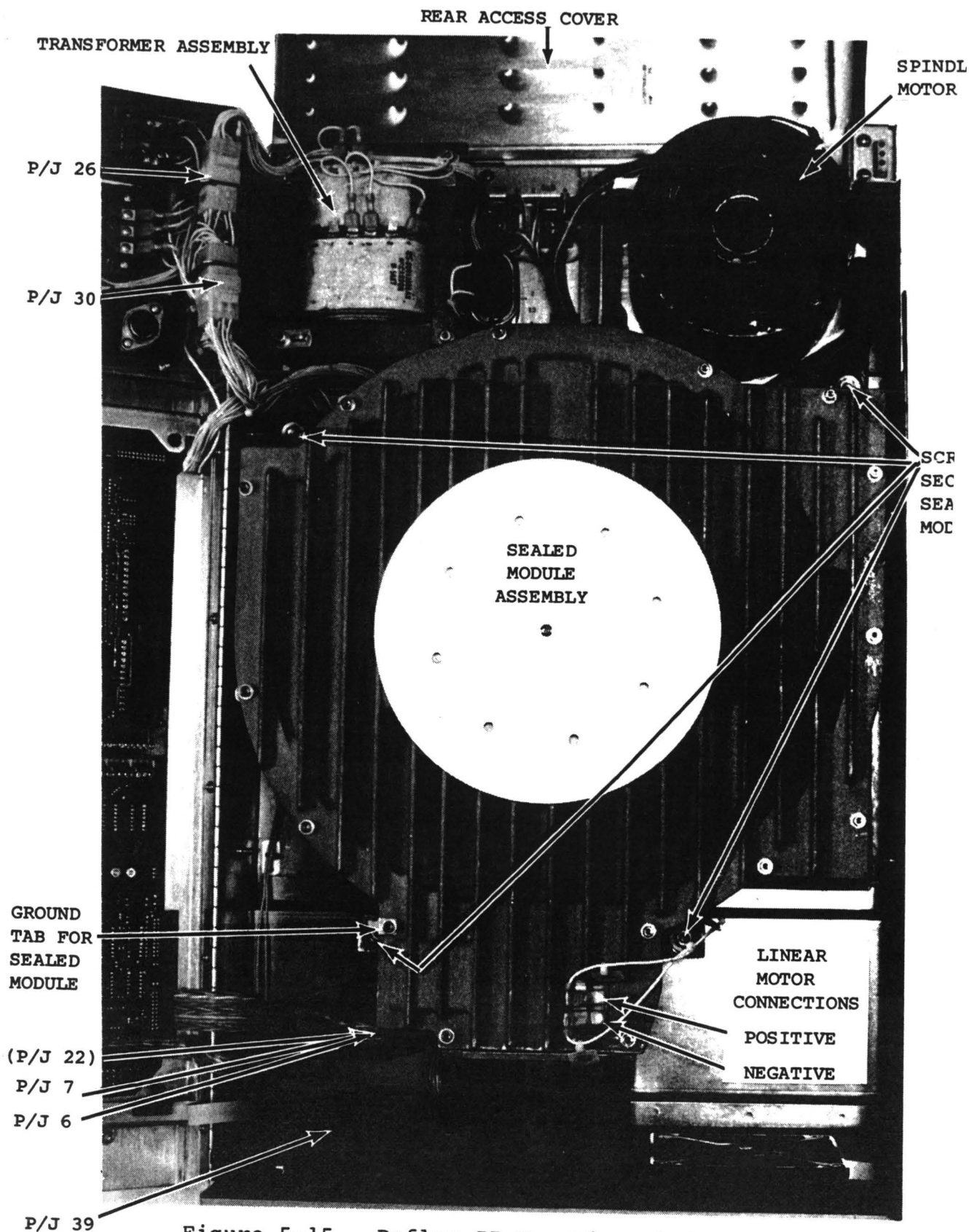
Figure 5-15. Reflex II Top View, Maintenance
