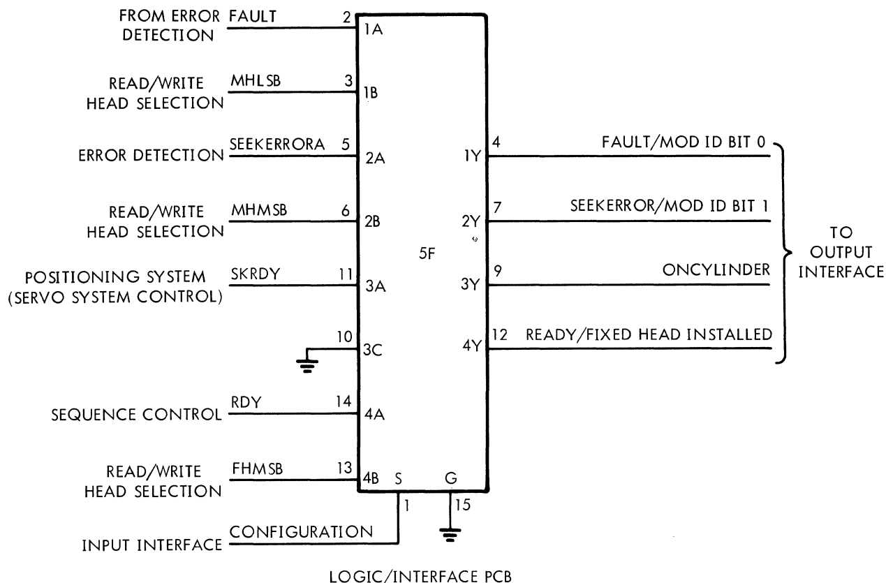
Figure 4-52. Primary/Alternate Status
