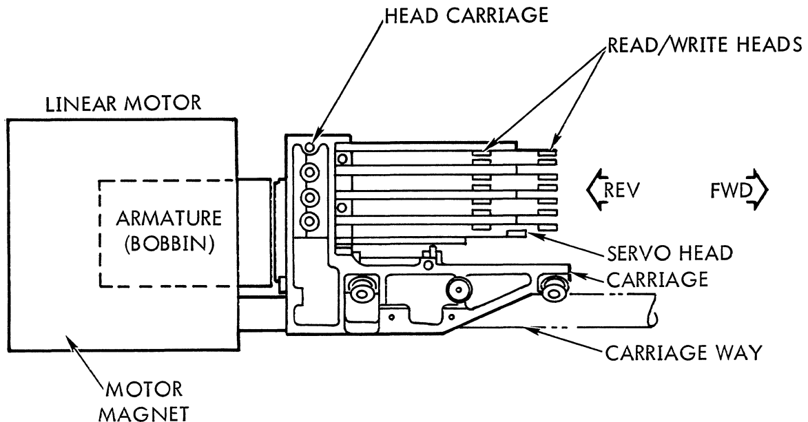
Figure 1-5. Positioner Mechanism
