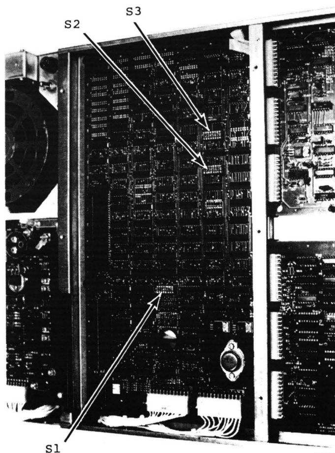
Figure 3-9. Logic/Interface Switches
