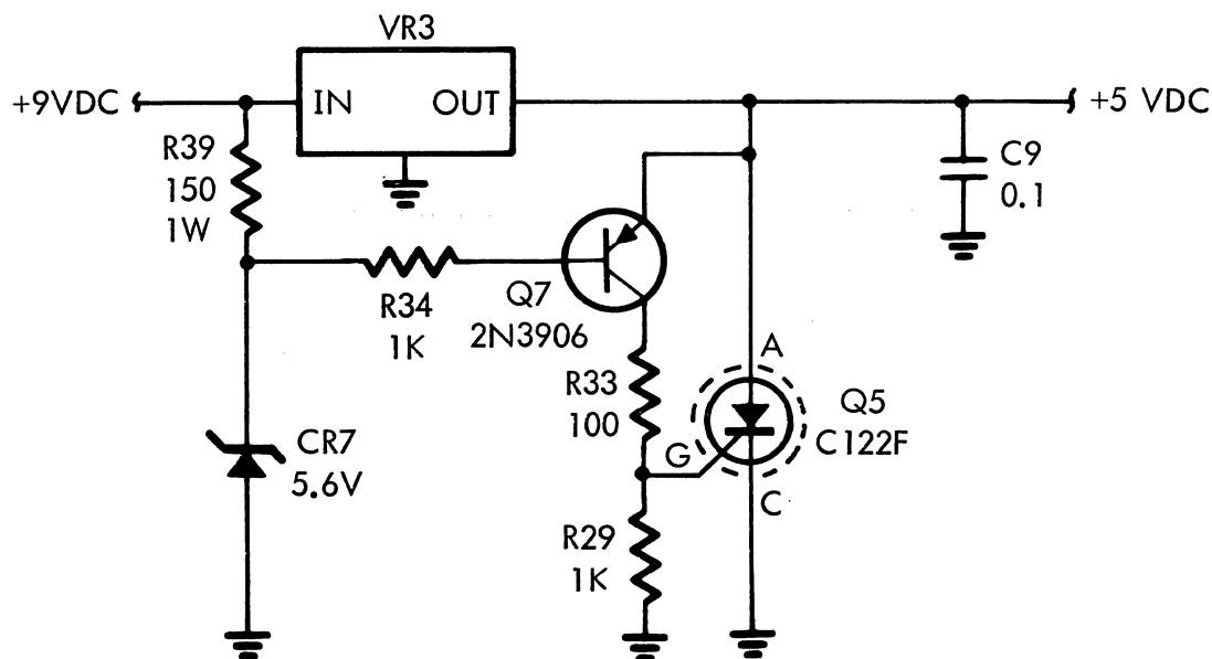
Figure 4-6. +5V Over Voltage Protection
