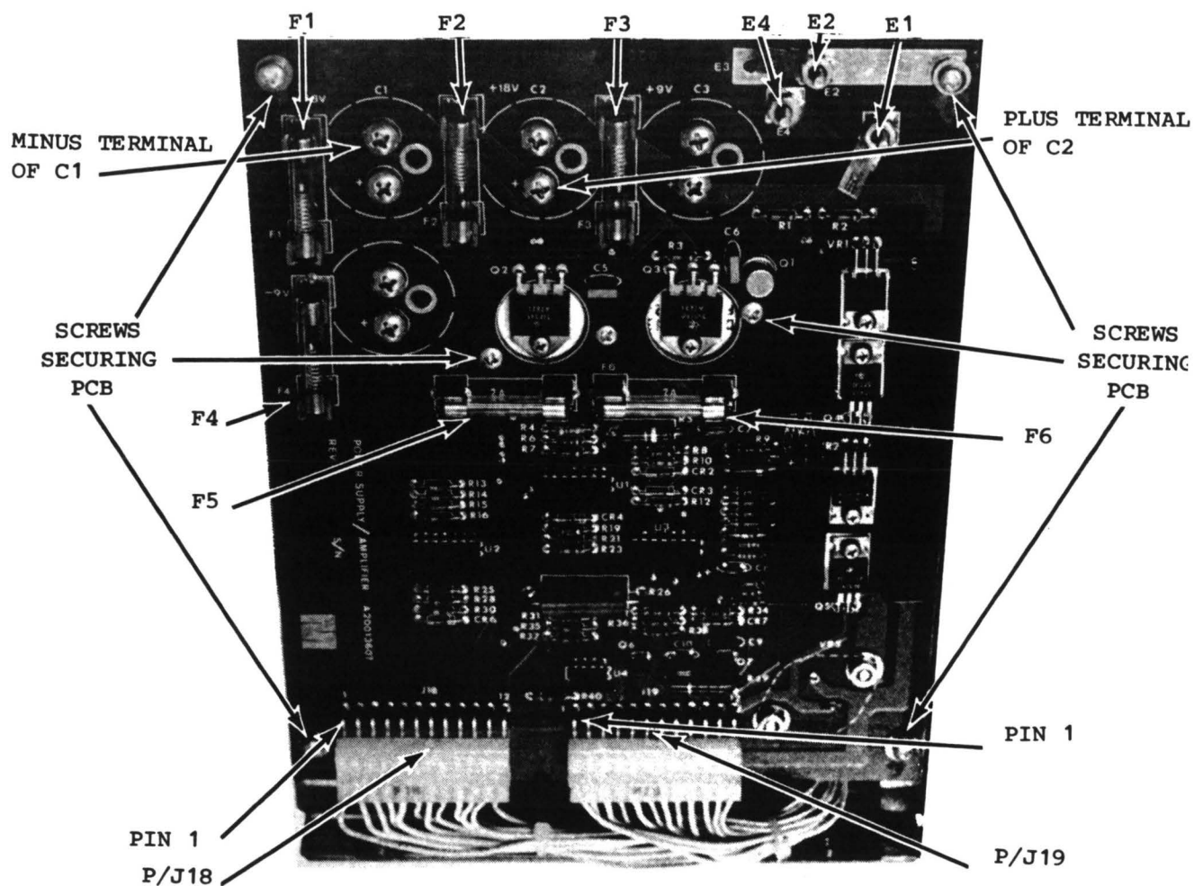
Figure 5-2. Power Supply/Amplifier PCB
