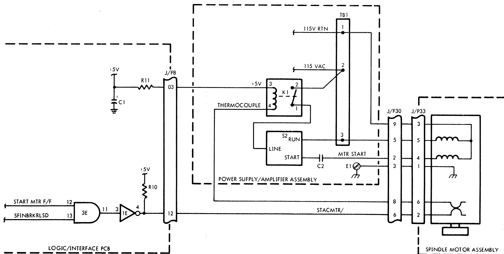
Figure 4-19. Spindle Motor Control
