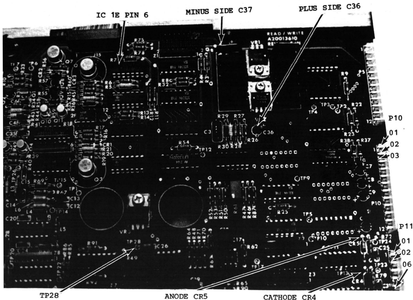
Figure 5-4. Read/Write DC Voltages
