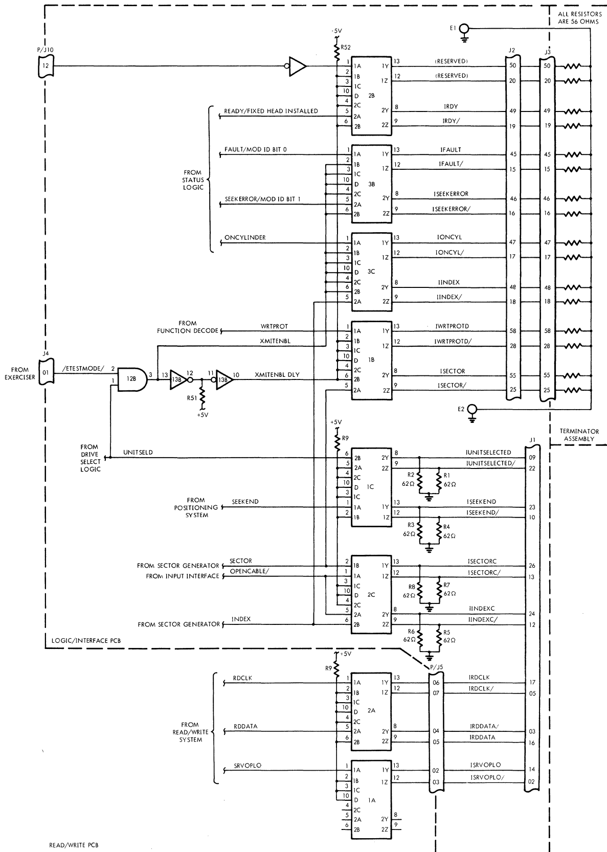
Figure 4-53. Output Interface
