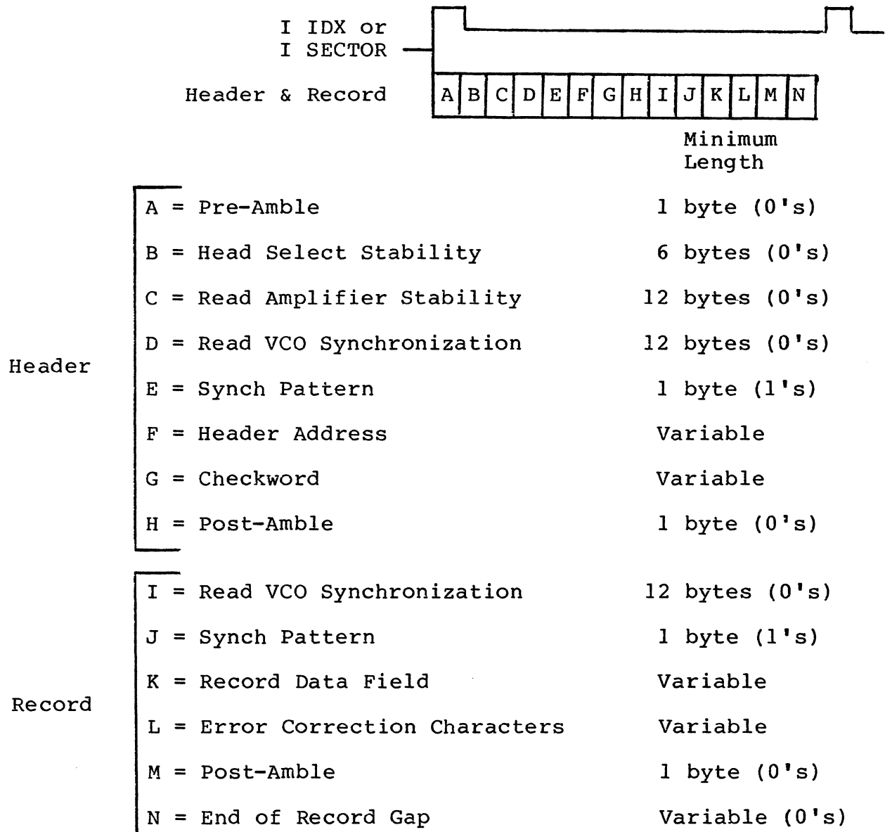
Figure 2-25. Format Summary
