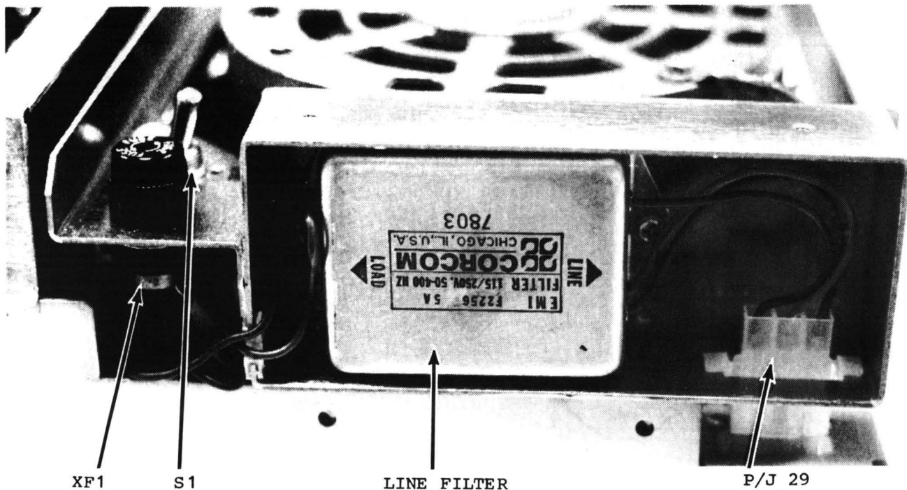
Figure 5-19. Line Filter Assembly
