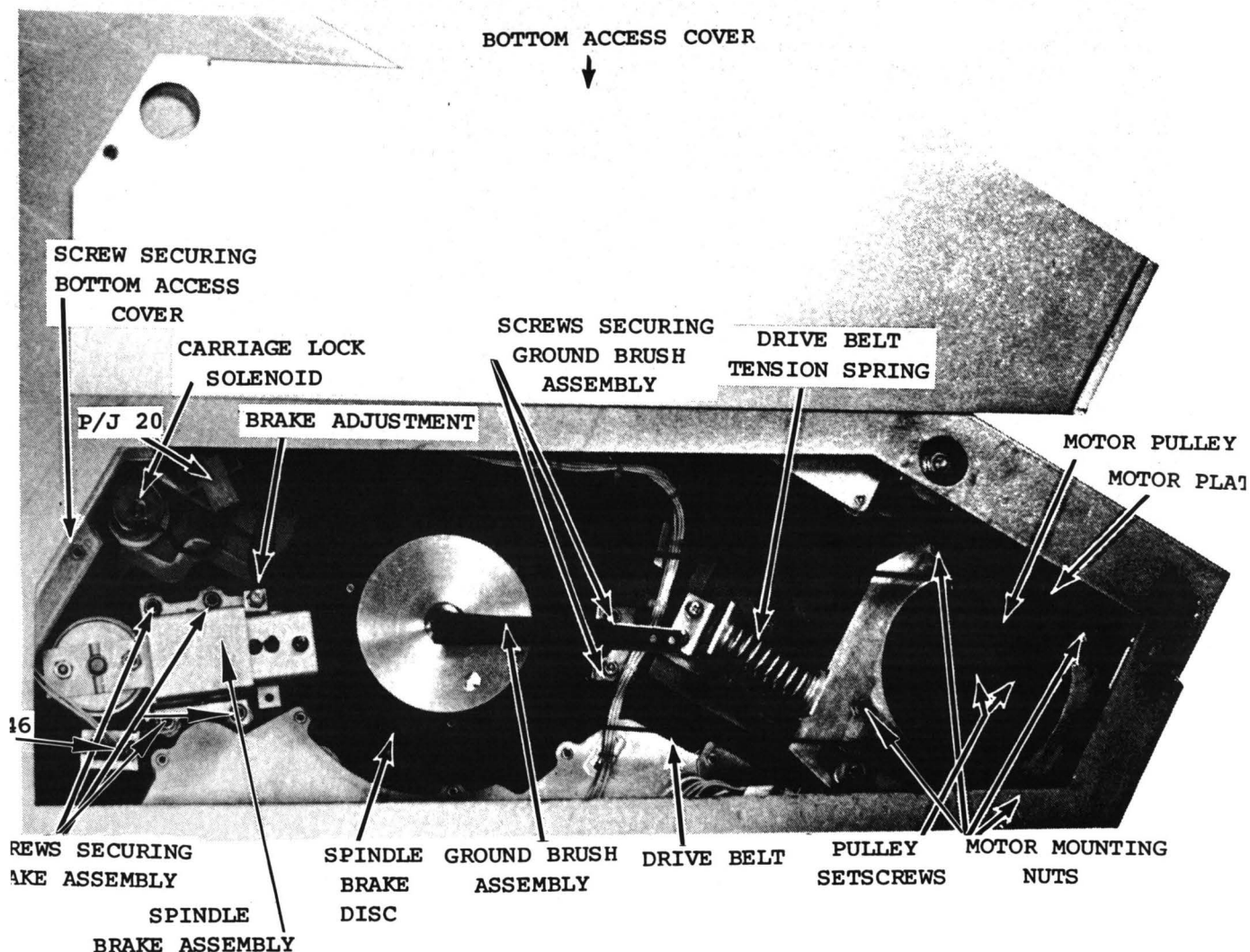
Figure 5-17. Reflex II Bottom View
