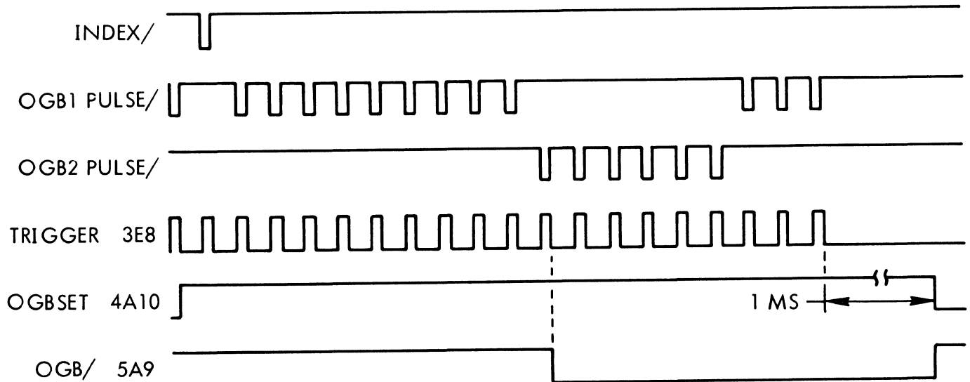
Figure 4-35. Outer Guard Band Detection
