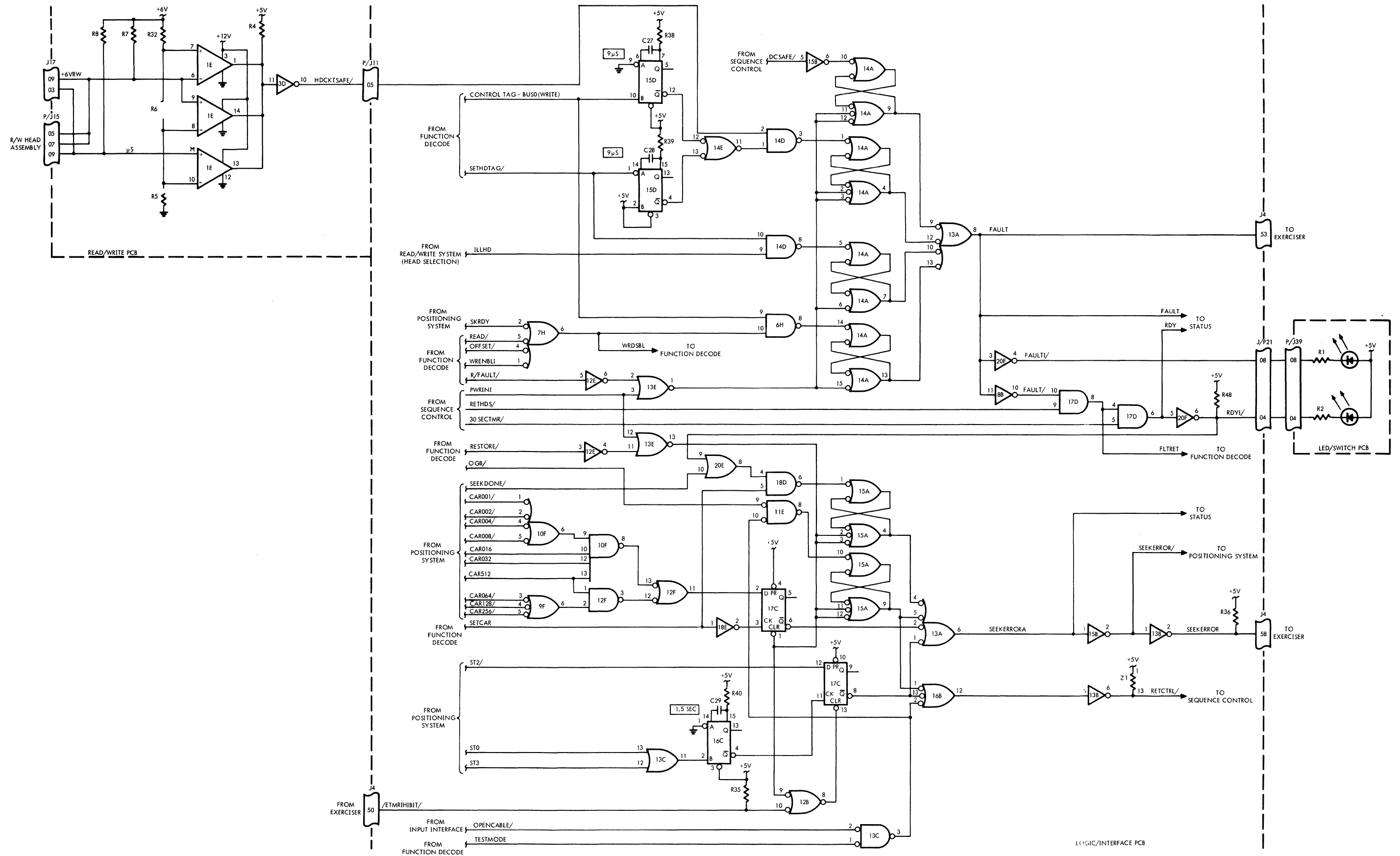
Figure 4-51. Fault Logic
