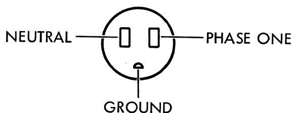
Figure 2-2. Standard AC Power Outlet Configuration
