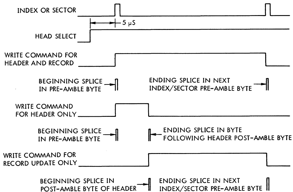
Figure 2-24. Splice Location
