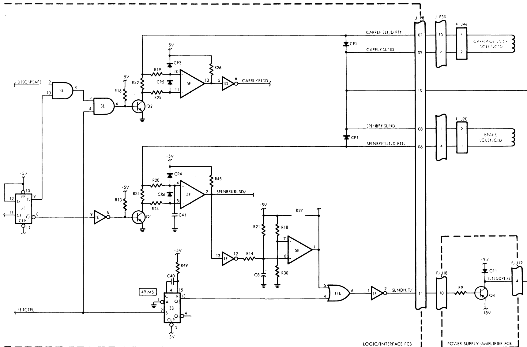
Figure 4-18. Solenoid Drive
