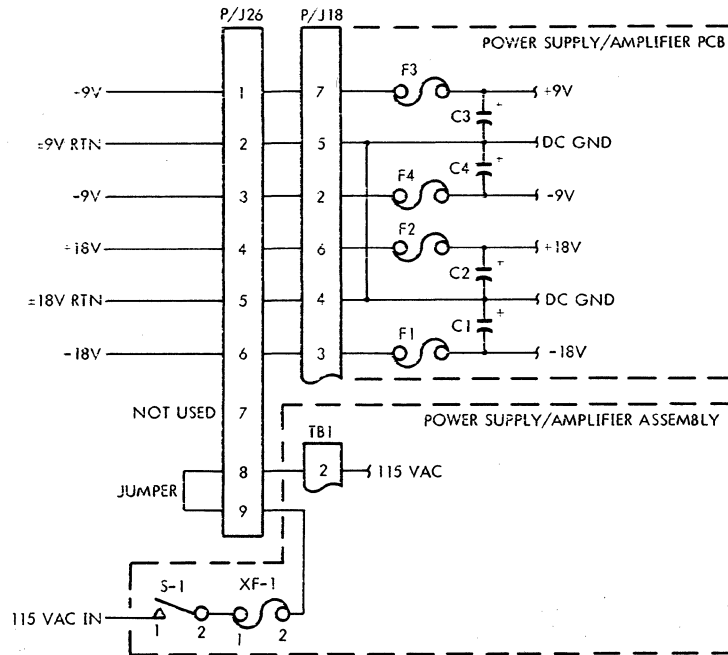
Figure 3-3. DC Voltage Connection
