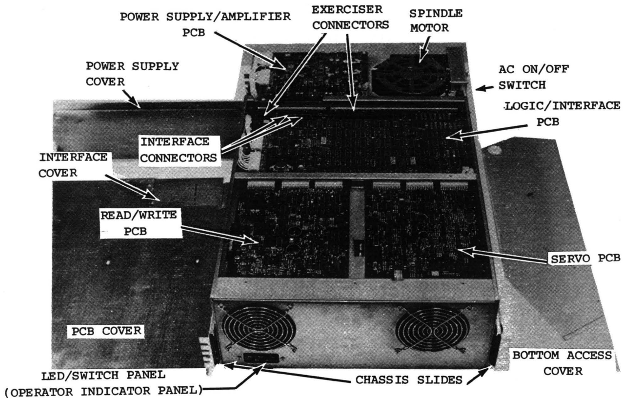
Figure 1-2. Reflex II Without Covers
