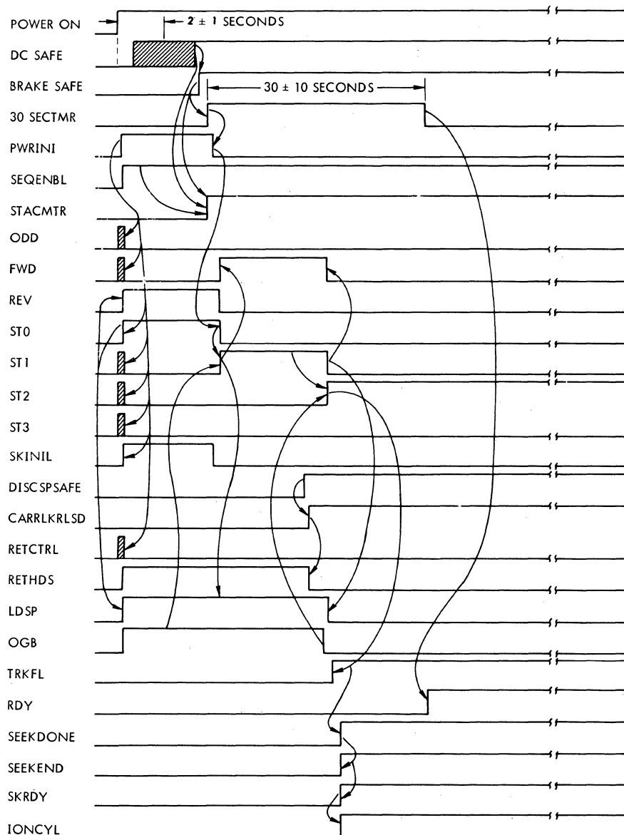
Figure 5-6. Sequence Up
