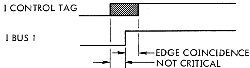
Figure 2-15. Read Command Timing
