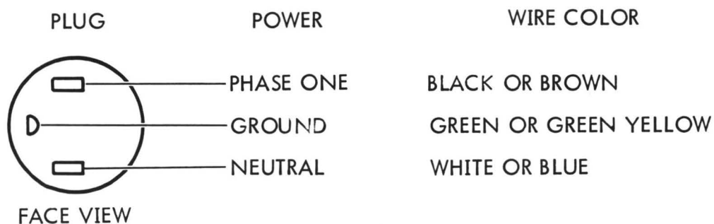
Figure 3-5. AC Power Cable Convention
