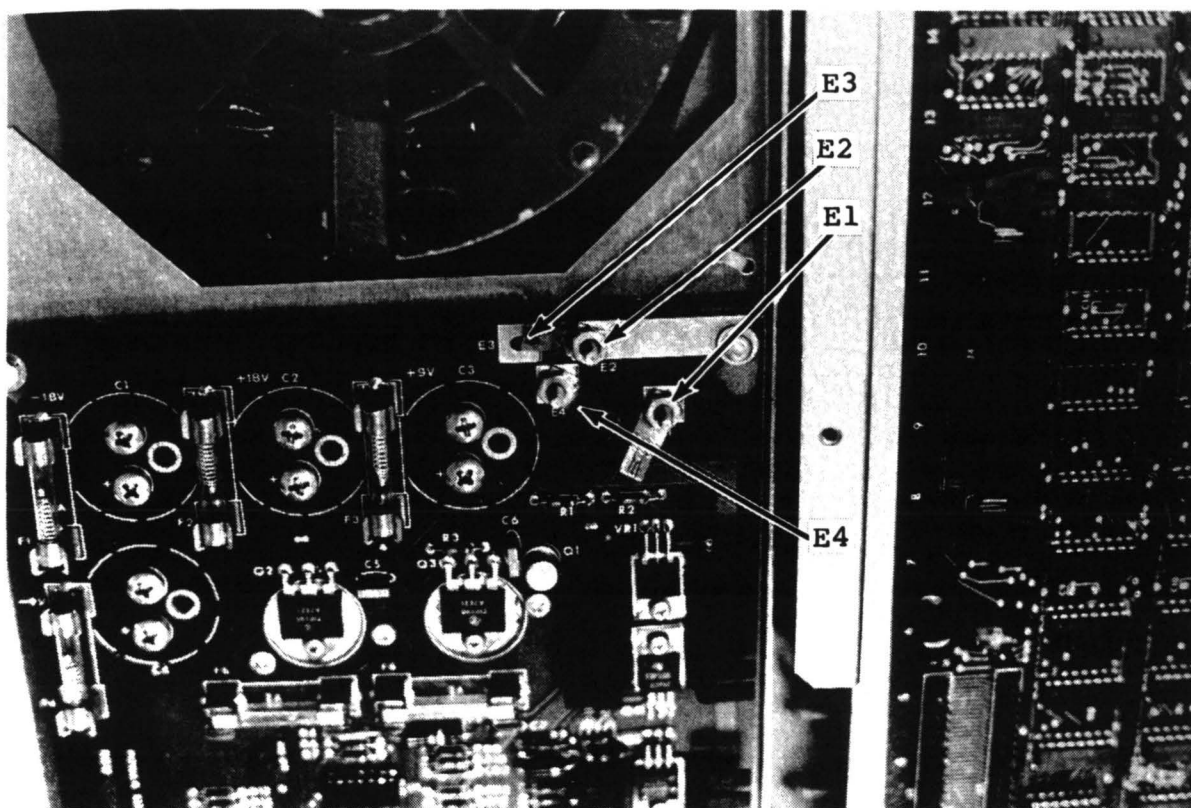
Figure 3-4. Ground Connection
