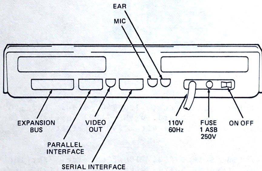
Rear of Sorcerer Computer
